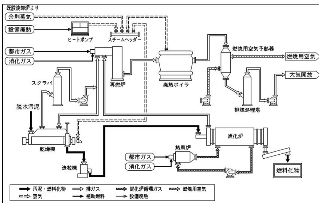
Fig. 1 Flow of sludge to fuel conversion
